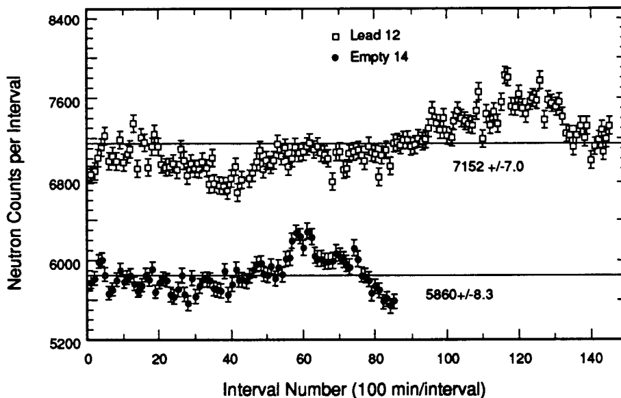
Fig. 11. Data obtained during the empty counter 14 and lead 12 runs. These data were obtained consecutively in the same aboveground location.
