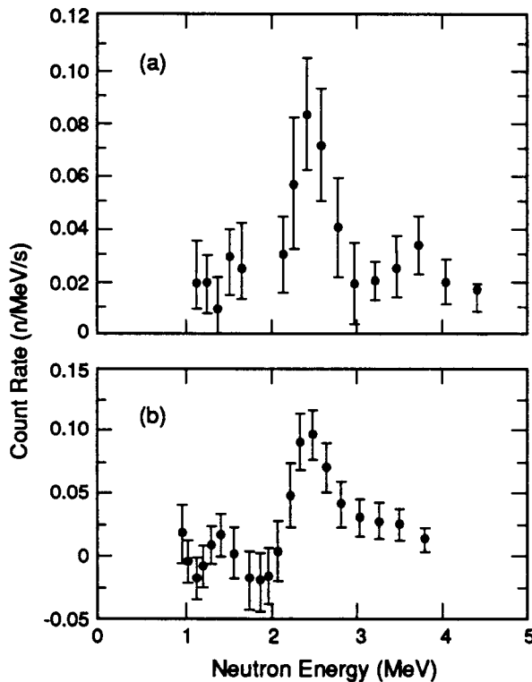
Fig. 12. (a) Spectrum of neutrons measured with an NE 213 counter during a 68-hr run. The data were unfolded from the measured spectrum based on measured response functions for monoenergetic neutrons. The bump near 2.5 MeV is about 3\sigma above background, but no excess count rate is present in the well counter data during the same interval. (b) Neutron spectrum measured with the NE 213 spectrometer but with no active cell present.
