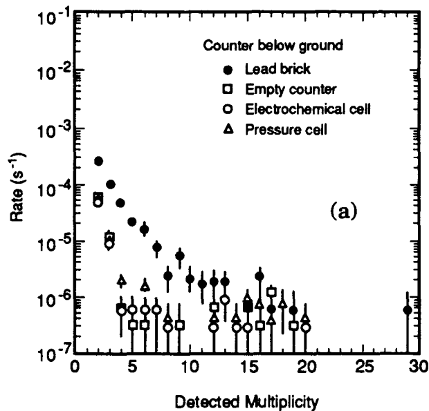
Fig. 10. Rates observed for the production of high-multiplicity events obtained (a) below ground and (b) aboveground. Events whose error bars reach 10^{-7} in the figure are due to one detected event, and hence the error bar actually reaches to zero. The multiplicity scaler overflows at 30 detected neutrons, and events of this size are not plotted in the figure. One such event was detected underground, and 22 such events were detected aboveground.
