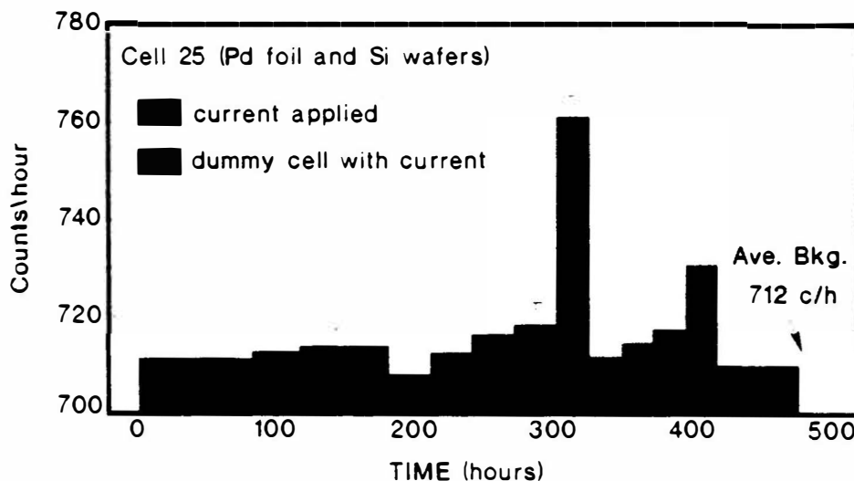
Figure 6. Neutron output from Cell 25 as a function of time. While not apparent because of the time scale, the cell output decayed as a function of time during operation.
