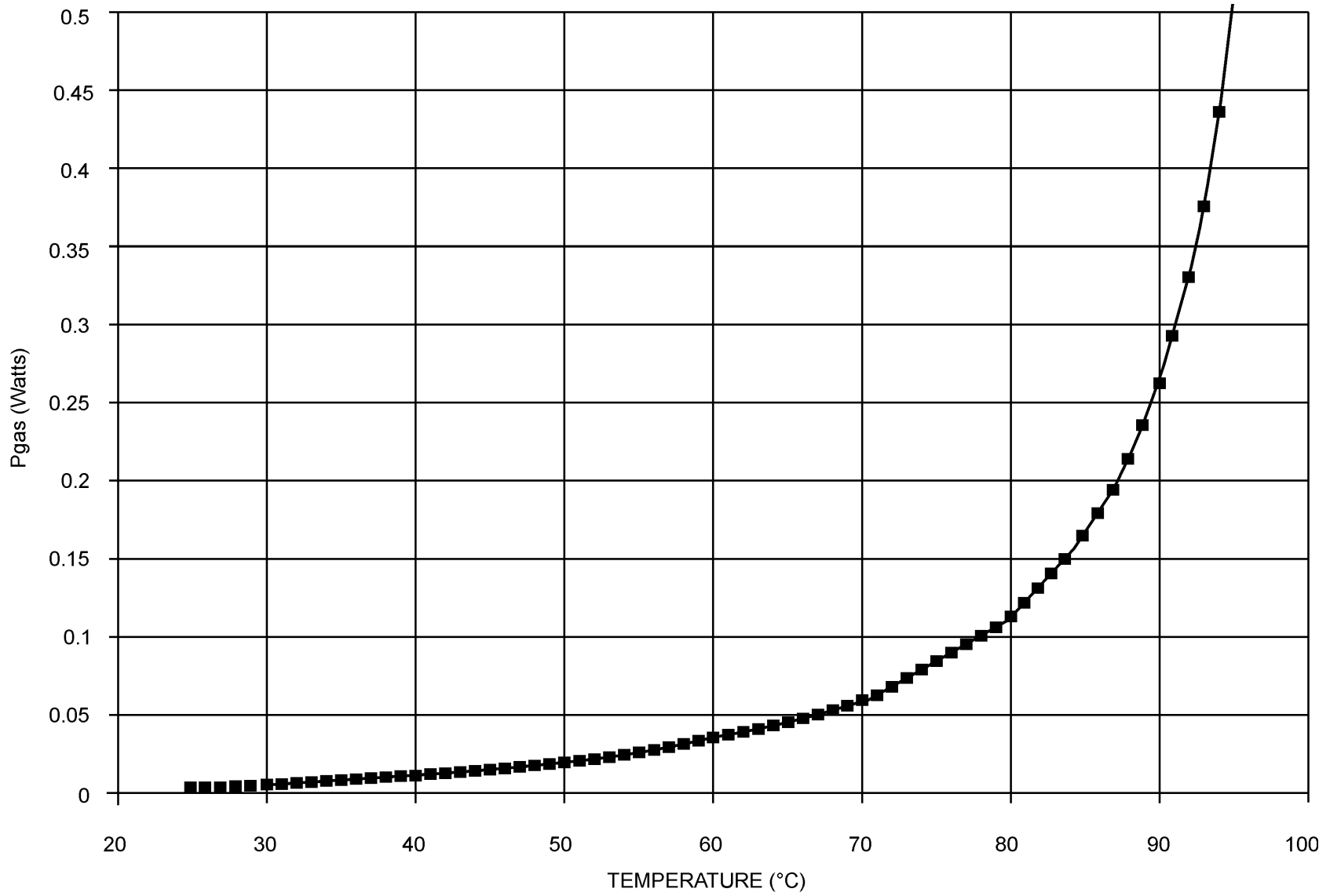
FIGURE 3. Theoretical Effect of the Cell Temperature on the P gas Term (Equation 2) When I = 0.500 A and the Bath Temperature is 27.50°C.
