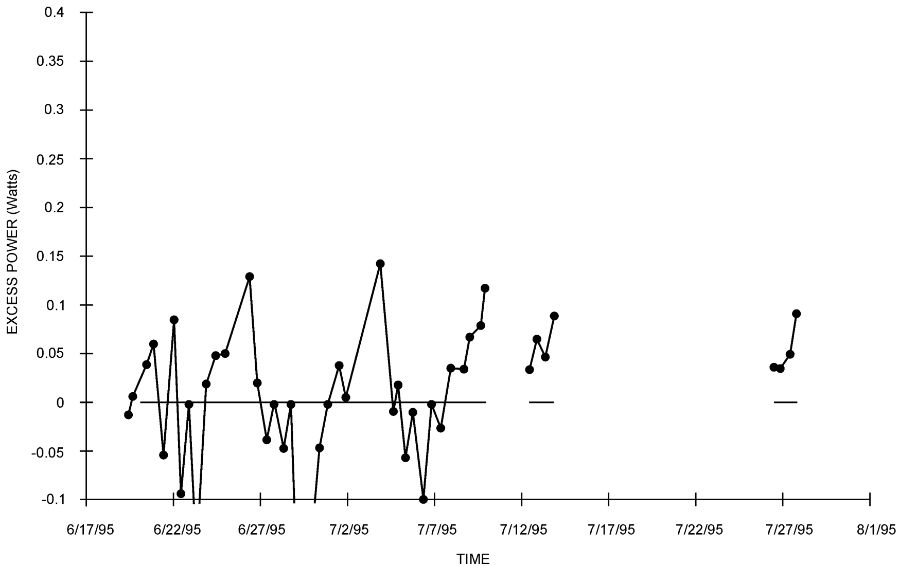
FIGURE 29. Excess Power Measurements for the Johnson-Matthey Palladium Wire (1 mm × 2.5 cm), Cell A. Calibrations following this experiment suggest no excess power.
