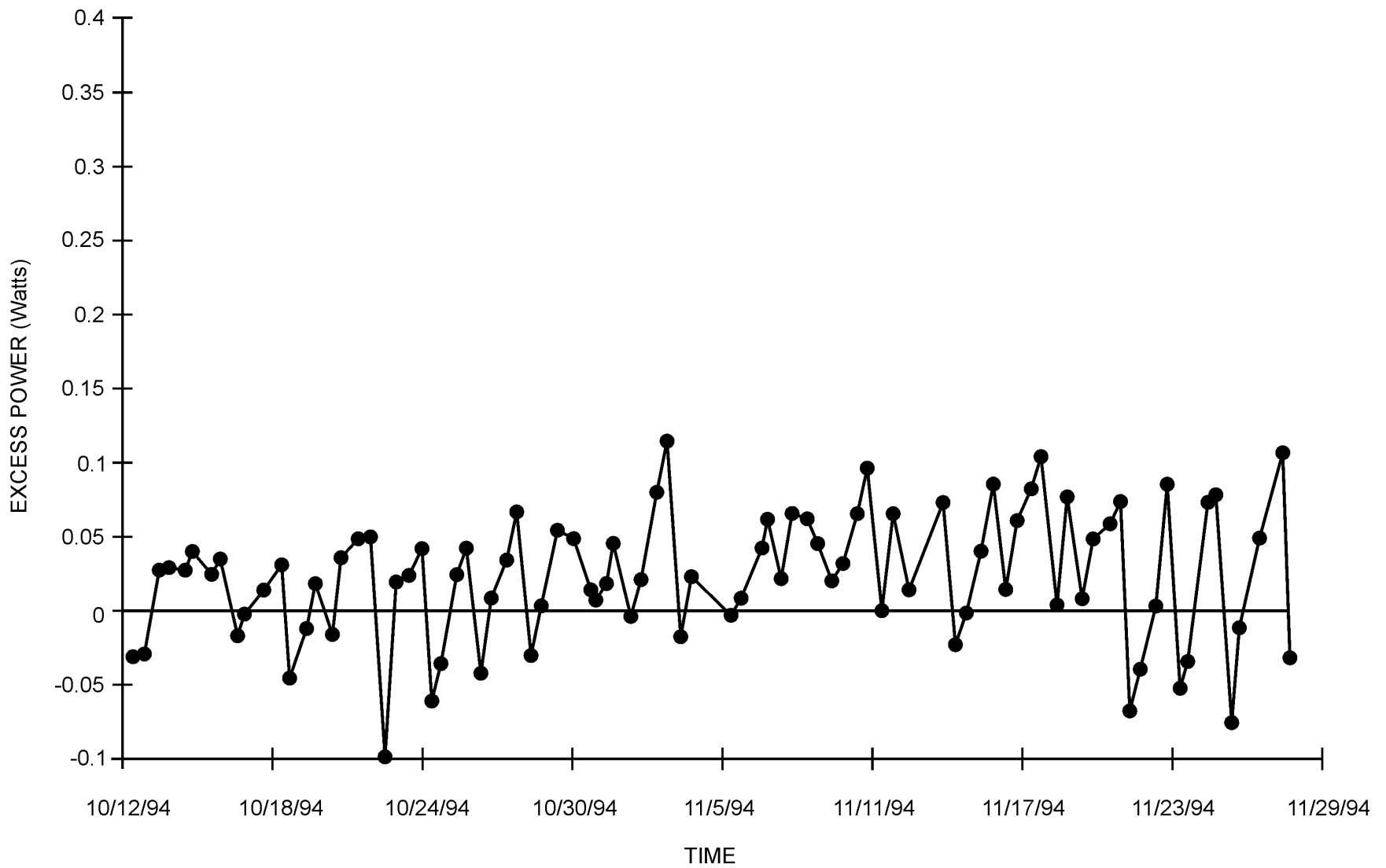
FIGURE 22. Experiment Showing No Significant Excess Power for an NRL Palladium-Boron Rod (2.5 mm × 2.5 cm, 0.75 weight % boron), Cell D. This rod contained a folded-over metal region that would act as a long crack.
