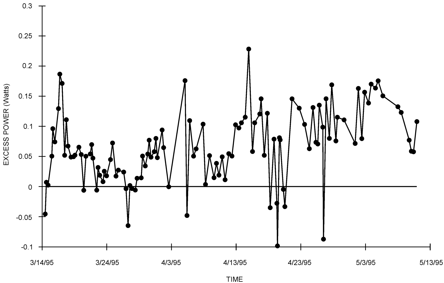
FIGURE 25. Excess Power Measurements for an NRL Palladium-Boron Rod (4.0 mm × 2.0 cm) Containing 0.25 Weight % Boron, Cell C. Typical excess power levels are 50-150 mW.
