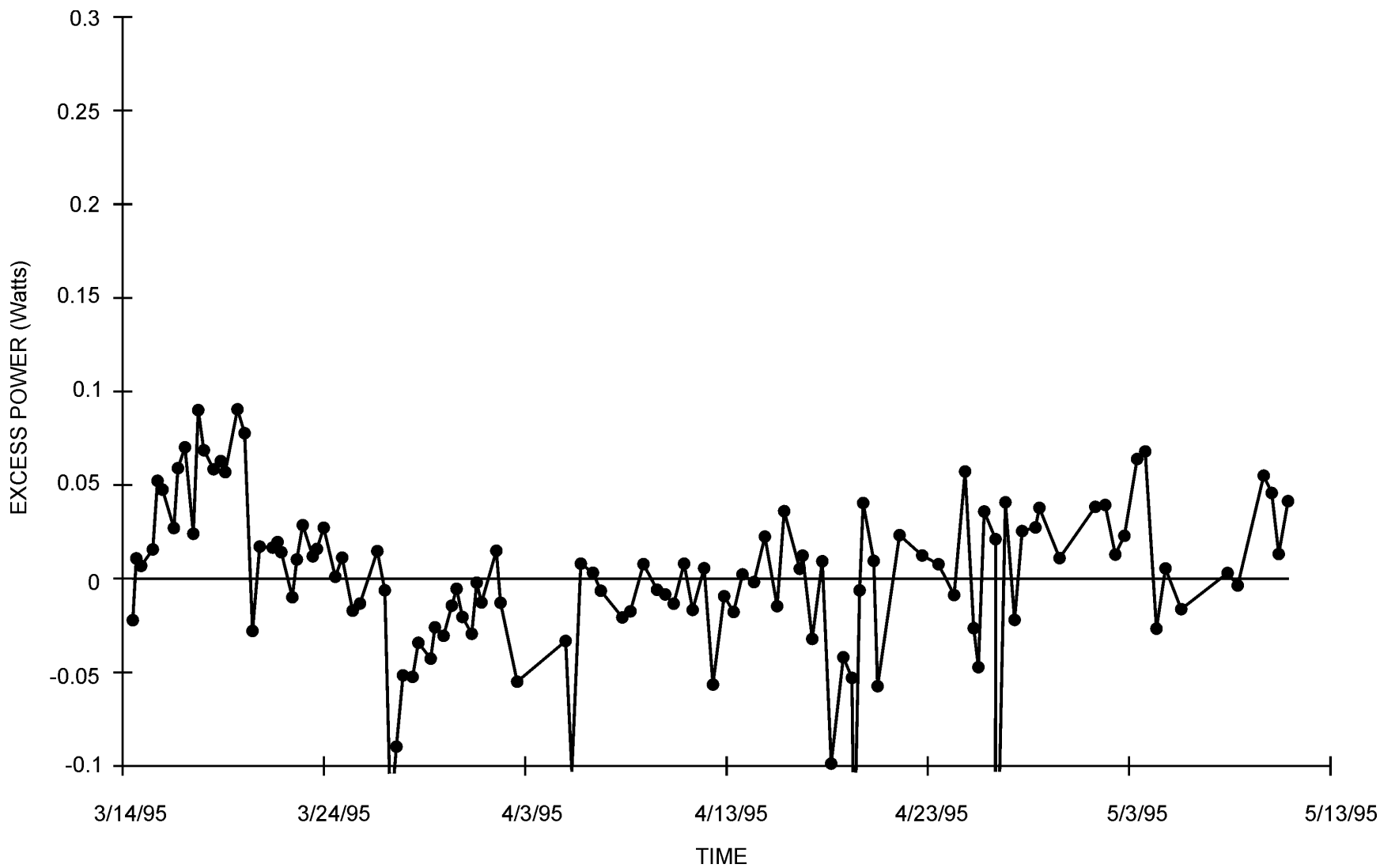
FIGURE 26. Excess Power Measurements for Another NRL Palladium-Boron Rod (4.0 mm × 2.0 cm) Containing 0.25 Weight % Boron, Cell D. A brief 5-day period of excess power was observed early in the experiment.
