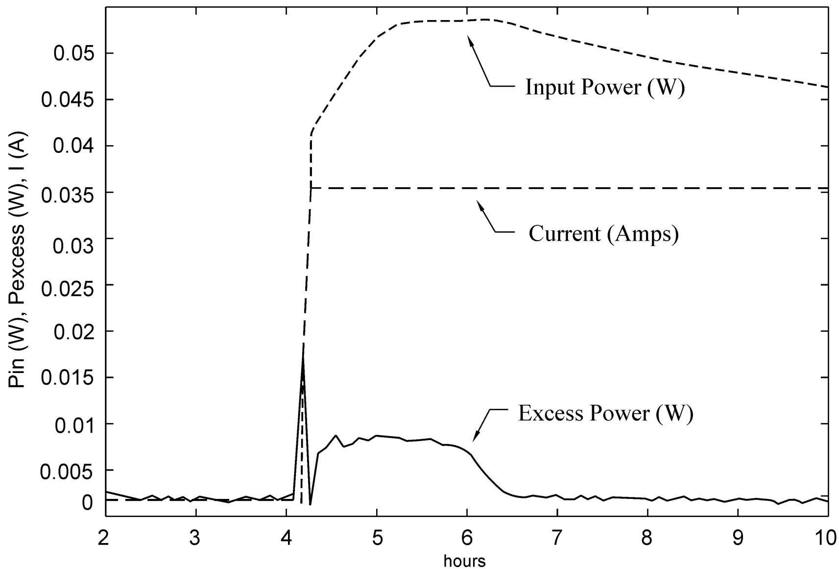
FIGURE 5. Measurement of the Exothermic Heat of Absorption of Deuterium Into a Palladium Wire (1 mm \times 4.3 cm) Using the New Calorimeter Developed at China Lake.
