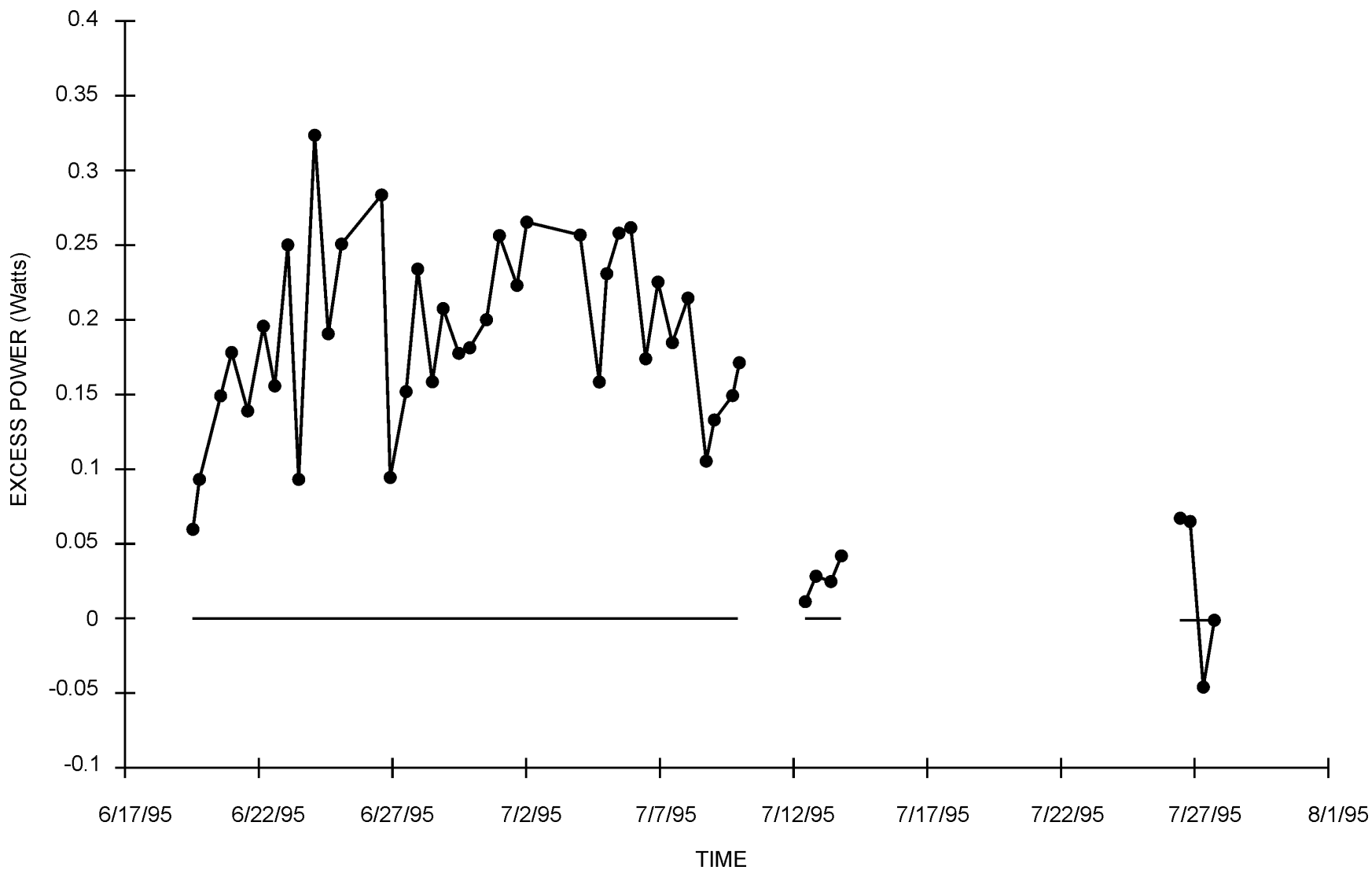
FIGURE 31. Excess Power Measurements for a Third Johnson-Matthey Palladium Wire (1 mm × 2.0 cm), Cell C. Significant excess power exceeding 200 mW was consistently observed. Calibrations checks following this experiment verify the excess power observations.
