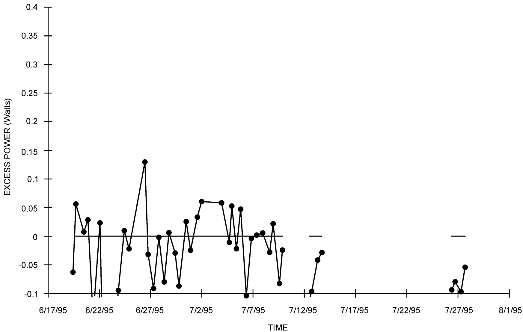
FIGURE 32. Excess Power Measurements for a Fourth Johnson-Matthey Palladium Wire (1 mm × 2.0 cm), Cell D. No significant excess power was observed. The calibration checks following this experiment, however, suggest a possibility of small excess power effects.
