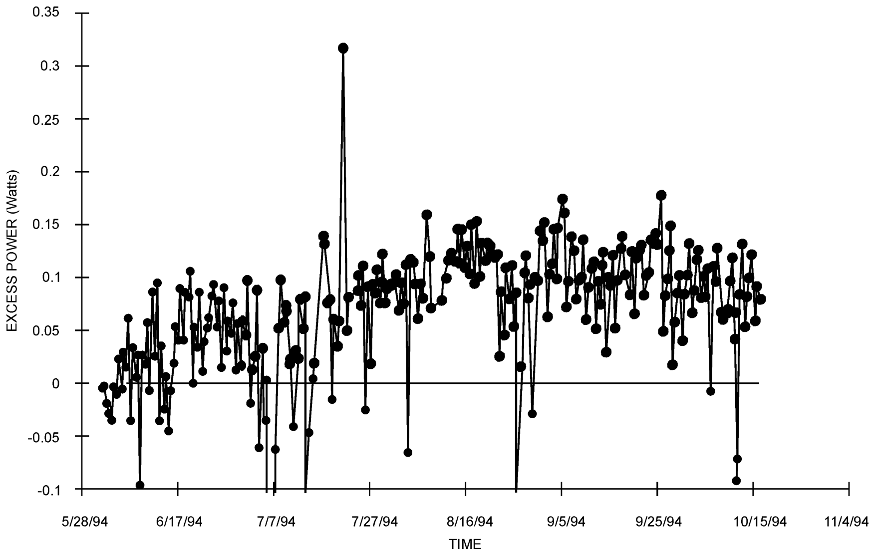
FIGURE 19. Excess Power Measurements for an NRL Palladium-Boron Rod (6.0 mm \times 2.0 cm, 0.75 weight % boron), Cell B.
