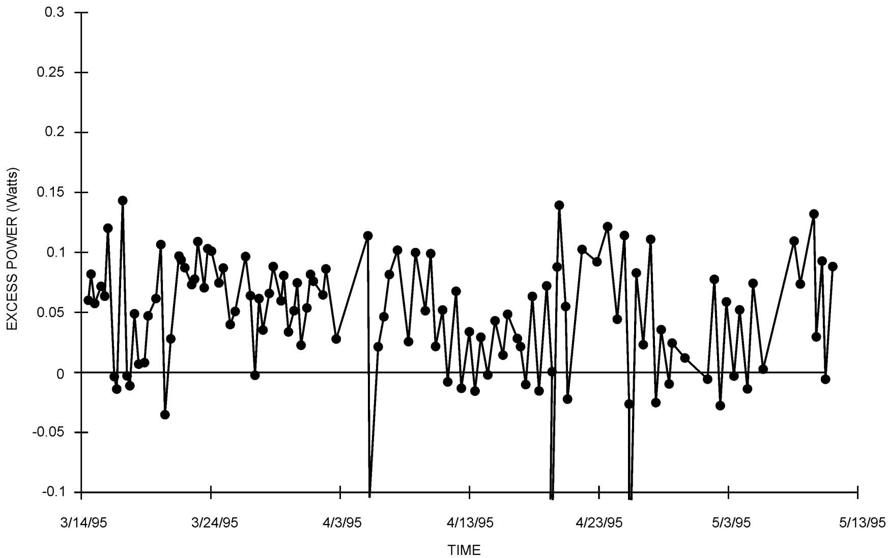
FIGURE 23. Excess Power Measurements for an NRL Palladium-Boron Rod (4.0 mm × 2.0 cm) Containing 0.50 Weight % Boron, Cell A. Excess power levels of 50-150 mW were observed.
