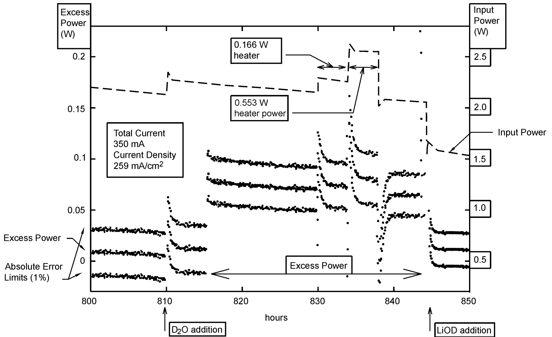
FIGURE 34. Excess Power Excursion for a 1-mm Johnson-Matthey Wire Cathode (1 mm × 4.3 cm) as Measured With the Improved China Lake Calorimeter. Excess power levels of approximately 75 mW are observed from 815 to 845 hours. Both the onset and the loss of the excess power effect were sudden.
