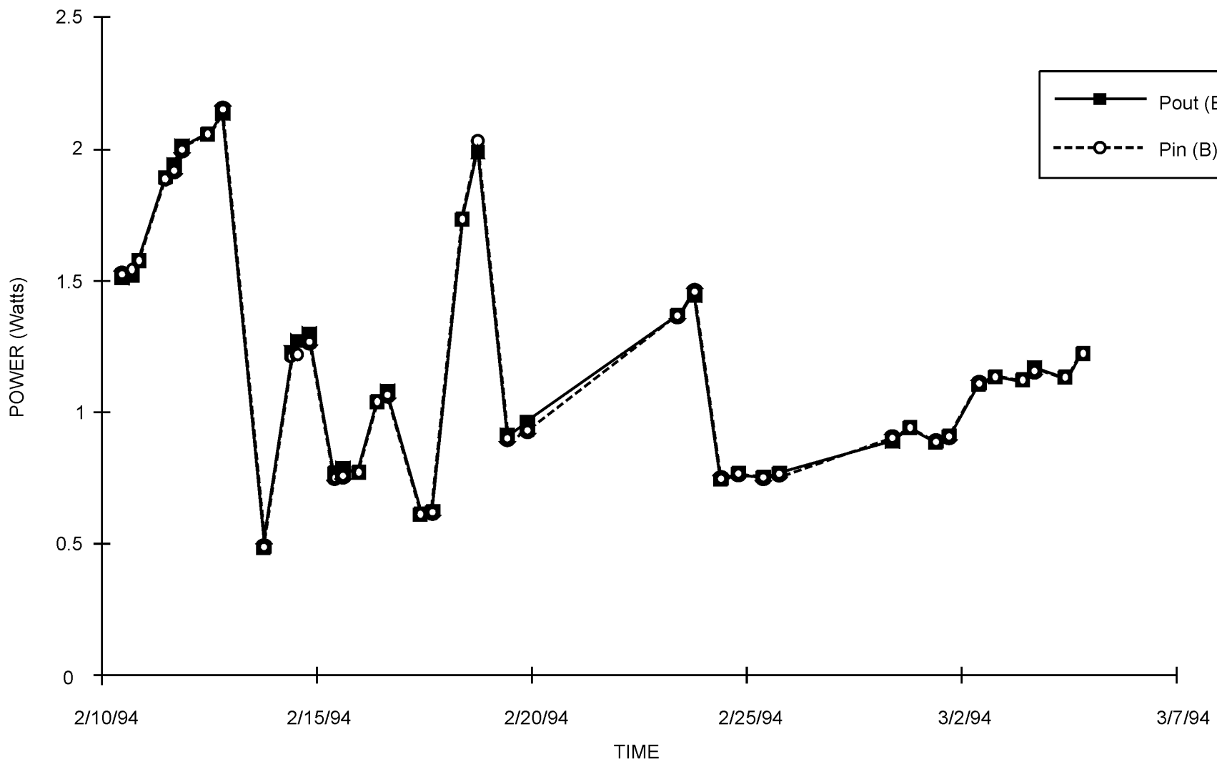
FIGURE 15. The Electrochemical Input Power and the Calorimetrically Measured Output Power for a Palladium Sheet Cathode Supplied by John Dash, Cell B. No excess power was observed.
