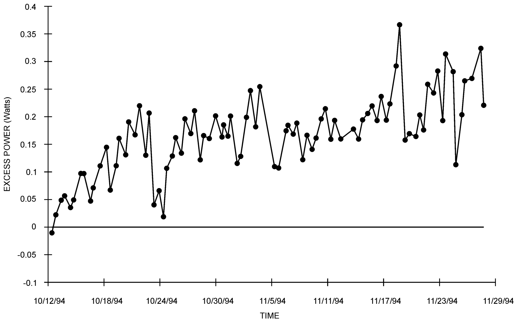
FIGURE 21. Excess Power Measurements for an NRL Palladium-Boron Rod (2.5 mm × 2.5 cm, 0.75 weight % boron), Cell C. A gradual increase in the excess power was observed. No flaws were visible for this cathode.
