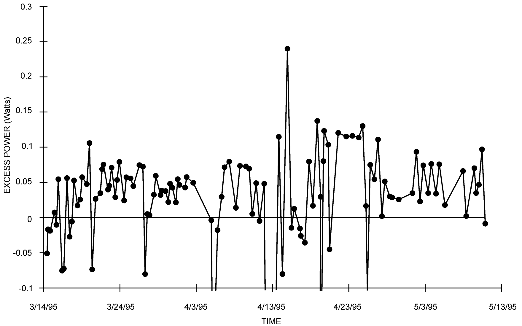
FIGURE 24. Excess Power Measurements for Another NRL Palladium-Boron Rod (4.0 mm × 2.0 cm) Containing 0.50 Weight % Boron, Cell B. Typical excess power levels are 50-150 mW.
