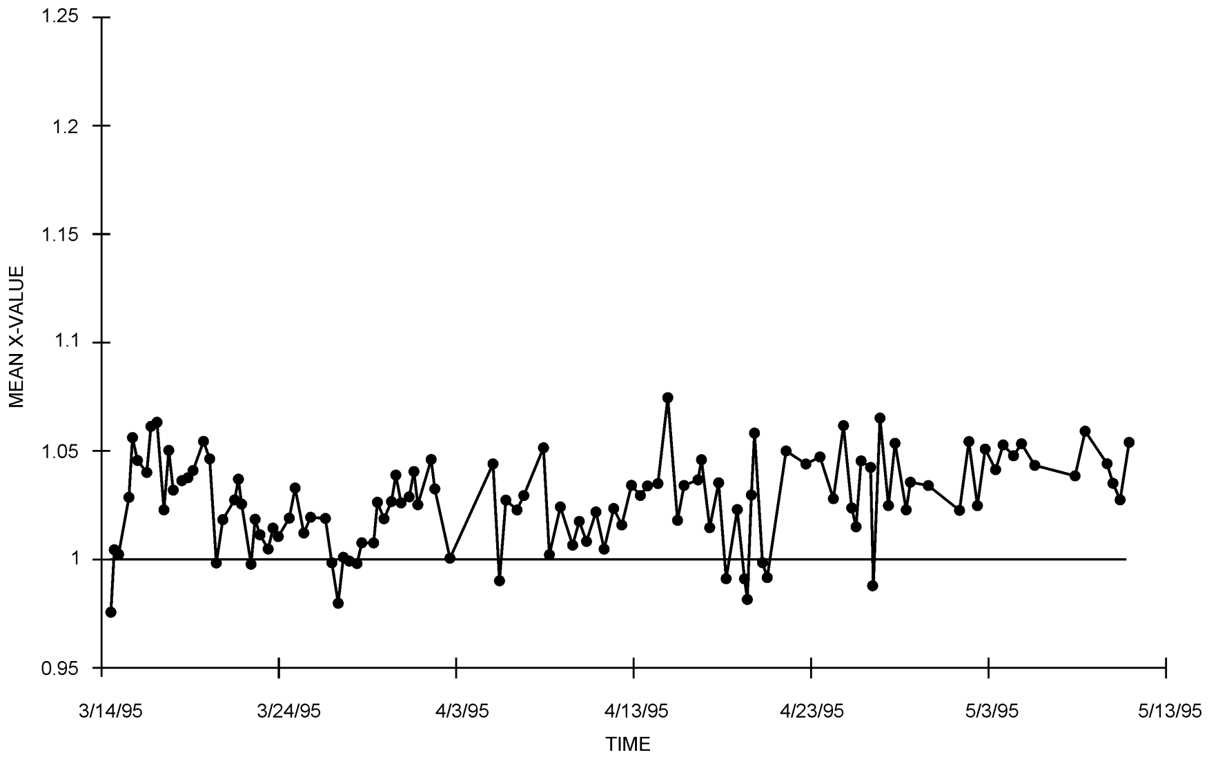
FIGURE 27. Ratio, X, of Output and Input Power for the Experiment Shown in Figure 25, Cell C.
