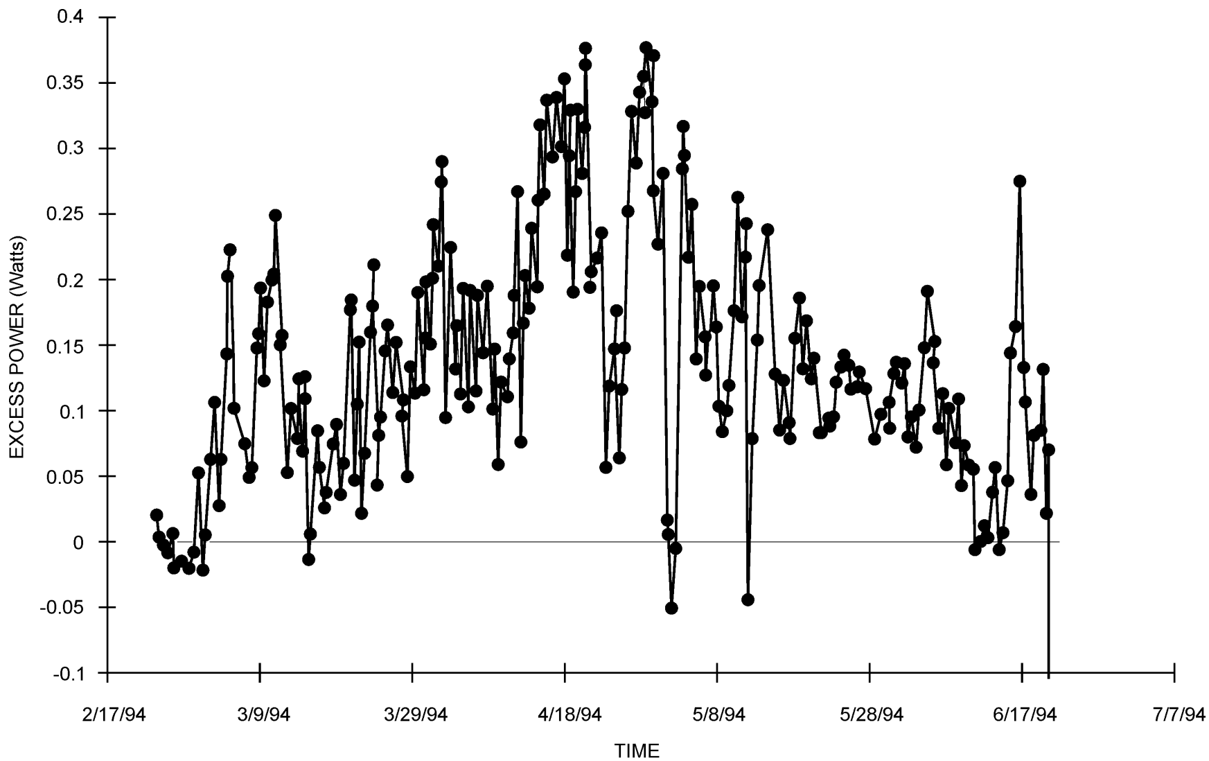
FIGURE 18. Excess Power Measurements for a Palladium-Cerium Alloy Rod (4.1 mm \times 1.9 cm) Obtained from Martin Fleischmann, Cell C. Excess power peaks of 350 mW were observed.
