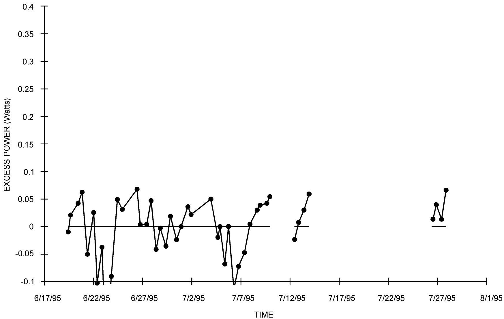
FIGURE 30. Excess Power Measurements for another Johnson-Matthey Palladium Wire (1 mm \times 2.5 cm), Cell B. No significant excess power was observed.
