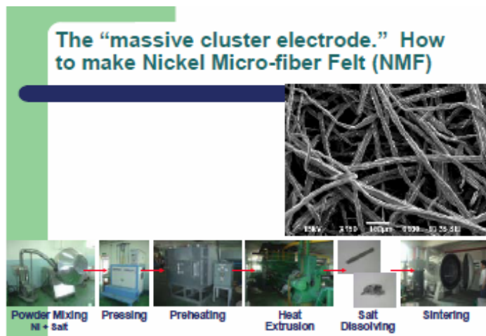
Figure 6. Construction steps for making Micro-fiber Felt (NMF) for the MCE.
